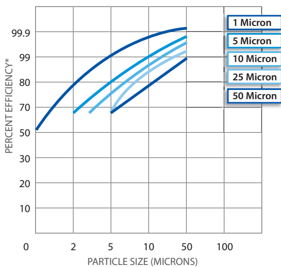
SPC Performance
