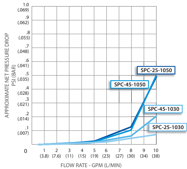
SPC Performance
