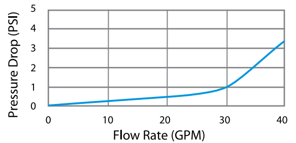
Pressure Drop
